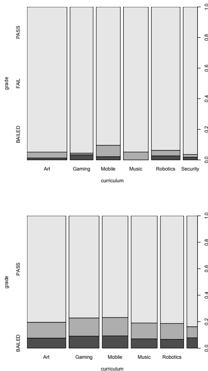
Figure 1: The top figure shows pass/fail rates for the various CS0 courses for the follow-on two programming courses for students with an AP computer science score. The bottom figure shows the same data but for students with no AP CS score. Dark grey shows the population that did not take a follow on course, mid-grey shows those who failed one of the courses and light grey, the majority, shows those who passed. The width of each bar corresponds to the number of students who took each flavor of CS0, for example, 466 students took the computational art flavor versus 136 students took security (a relatively new offering).
